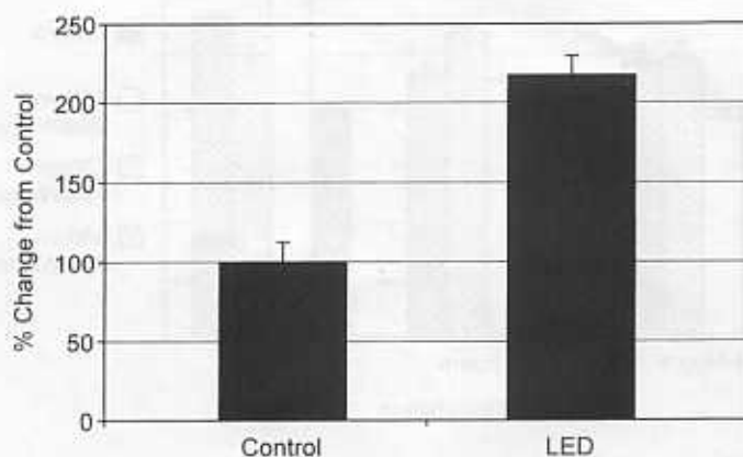
FIG. 6. HaCAT epithelial cell collagen synthesis at 8 J/cm², 50 mW/cm², 670 nm. Shown in 24-h 3 H proline incorporation.
